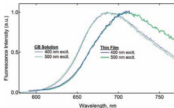
Figure 5. Steady-state fluorescence emission spectra of PCDTBT in chlorobenzene solution (dotted lines) and as a thin film (solid lines) after excitation at 400 nm (blue) or 500 nm (green).
